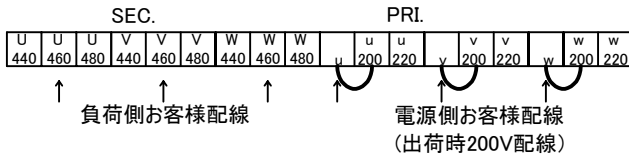
端子台配列 Terminals Arrangement
